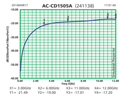
AC-CD1505A
