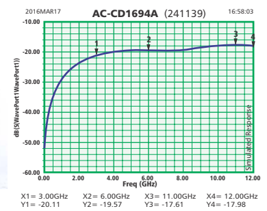
AC-CD1694A
