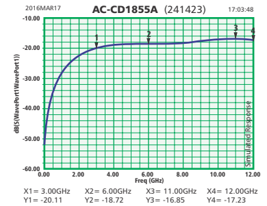
AC-CD1855A
