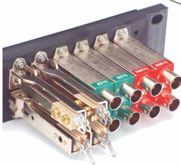
Longframe panels also accept AVP standard size video jacks
